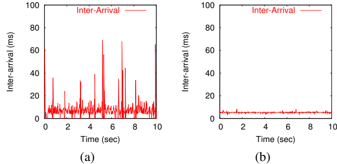
Fig. 6. Inter-arrival time of the packet pairs at the receiver: (a) Home (cable) to USC. (b) Home (ADSL) to USC.
