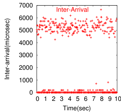
Fig. 11. An example of the packet-pair inter-arrival time of a dialup connection: the small median value might be due to traffic shapping.
