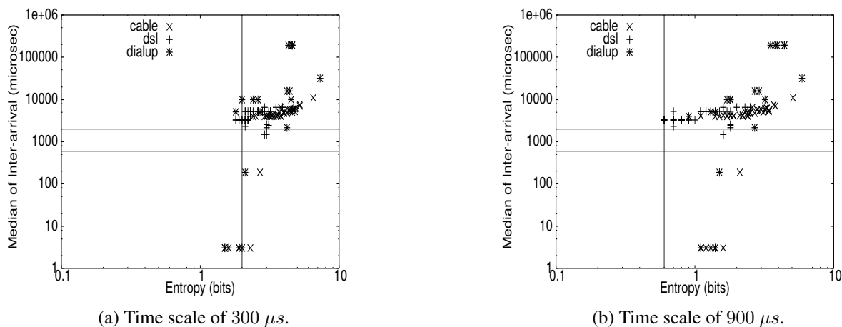
Fig. 10. Large-scale uncontrolled experiments: classification results for connection types of cable, ADSL and dialup (UMass-1 as the receiver).
