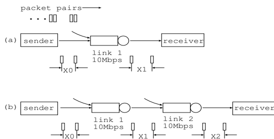
Fig. 3. Settings for the analysis: one and two 10 Mbps links connect the sender and the receiver in Setting (a) and (b) respectively.
