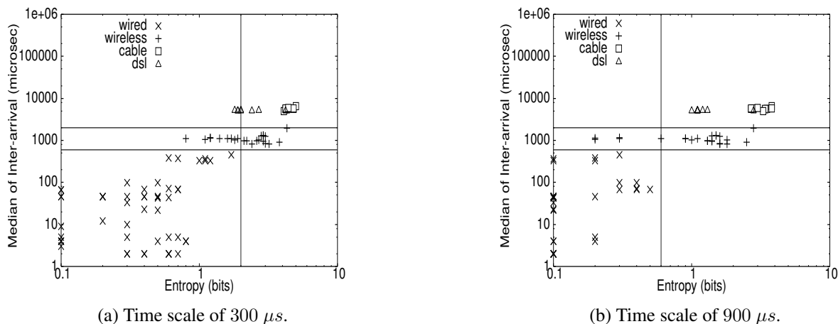
Fig. 7. Small-scale controlled experiments: classification results.
