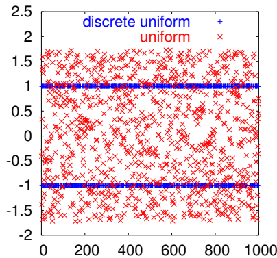
Fig. 1. Two distributions with the same mean, variance but very different entropy.
