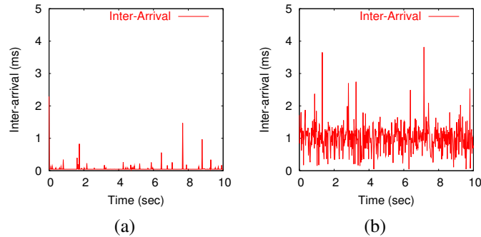
Fig. 5. Inter-arrival time of the packet pairs at the receiver: (a) UMass (Ethernet) to USC. (b) UMass (WLAN) to USC.
