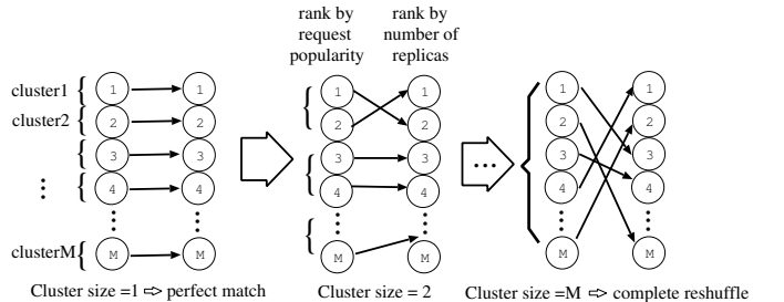
Fig. 9. Clustered shuffling to create mismatch between file ranks
